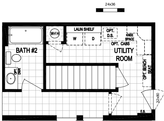
OPTIONAL BASEMENT STAIRWELL #2 (OMITS THE FURNACE)
