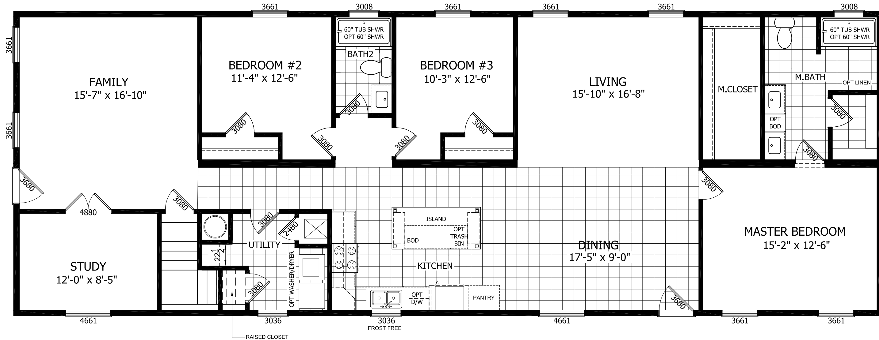
HEM 2876-3D - 1 3 BEDROOM / 2 BATH
